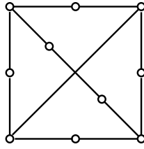
Figure 3.1: A non-h-perfect graph whose clique- and odd-hole-acyclic superorientations all have kernels
